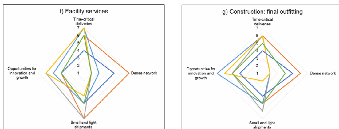
Figure 4 Multi-criteria evaluation
